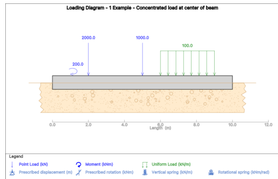
Figure 3 Loading Diagram
